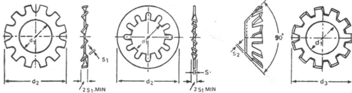
Type A: Externally Toothed T
